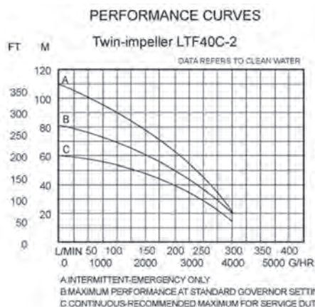
LTF40C-2 (2 IMPELLER)
